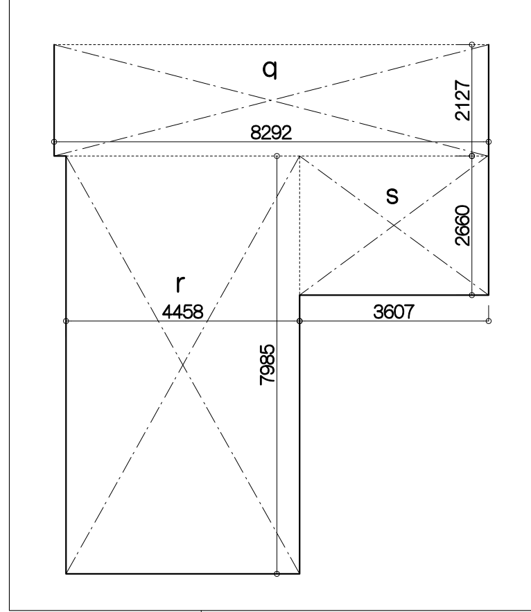
別図A：②-q,r,s(S:1/100 A1)
